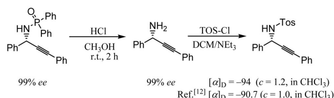
Figure 2. Determination of the absolute stereochemistry of N -(1,3-diphenylprop-2-ynyl)- P,P -diphenylphosphinic amide. The literature value is from ref. [12]
